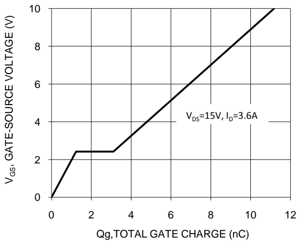
Figure 11. Gate Charge
